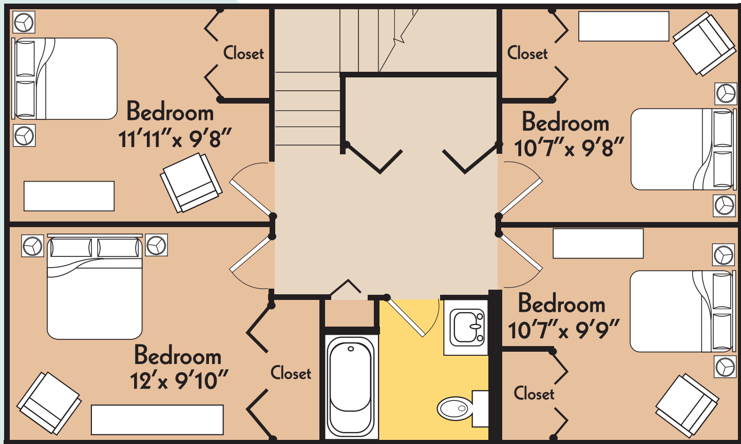
THE ANCHOR • SECOND FLOOR PLAN • 4 BEDROOM
