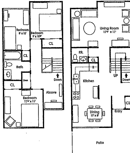
Three Bedroom Townhouse with Basement 1,782 Sq. Ft.
