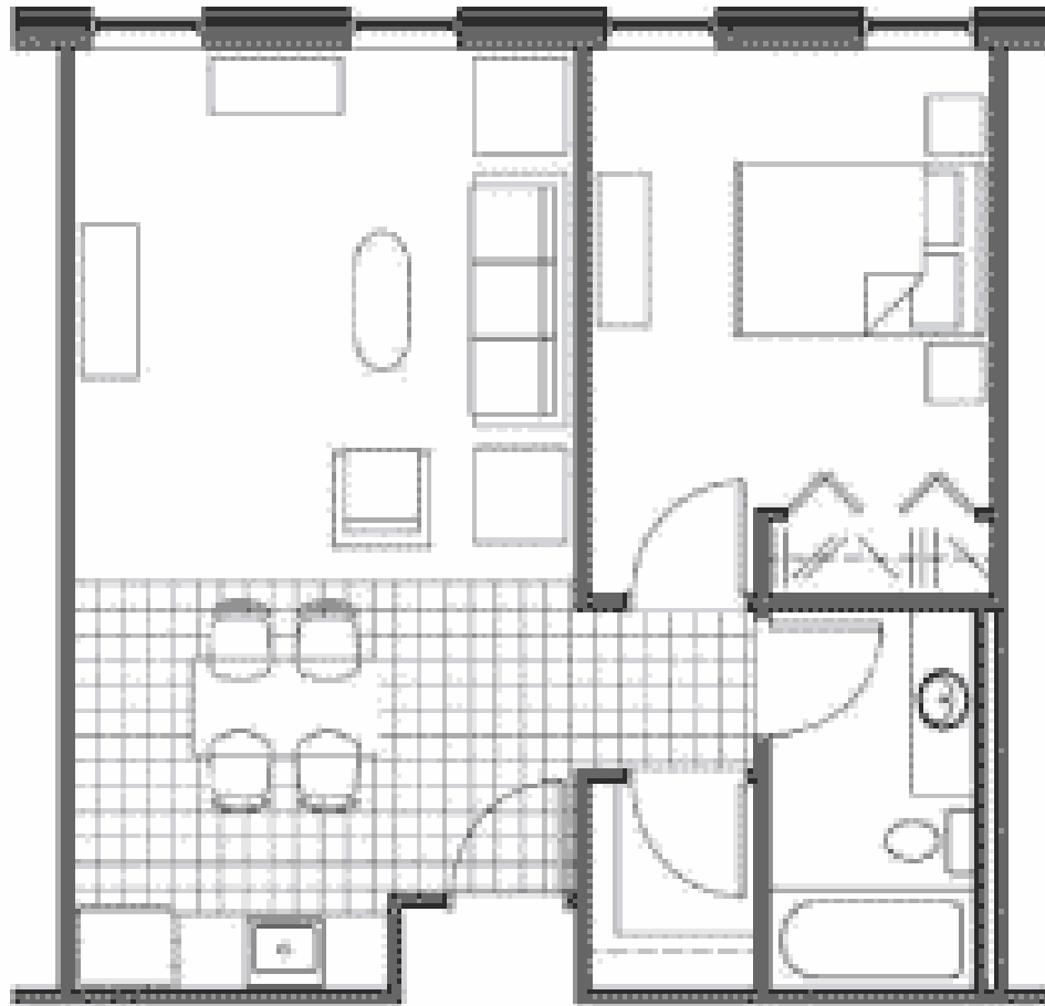
1 BR LIVING UNIT PLAN
