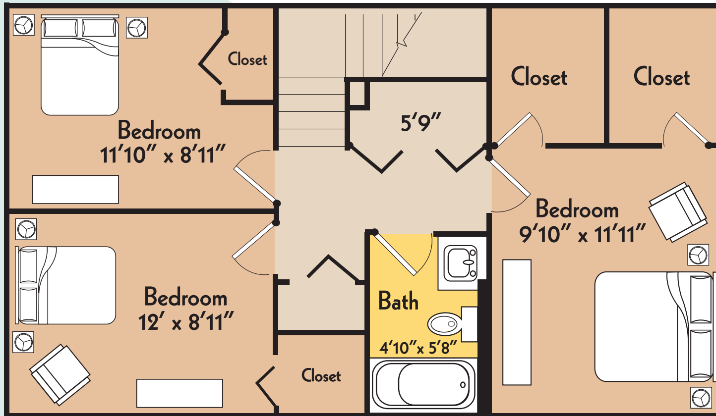
THE TIDE • SECOND FLOOR PLAN • 3 BEDROOM
